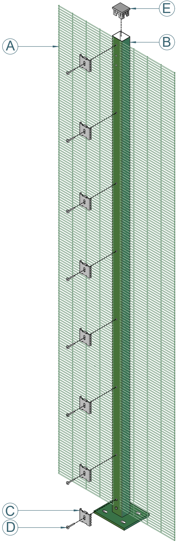
Axonometric Drawing
