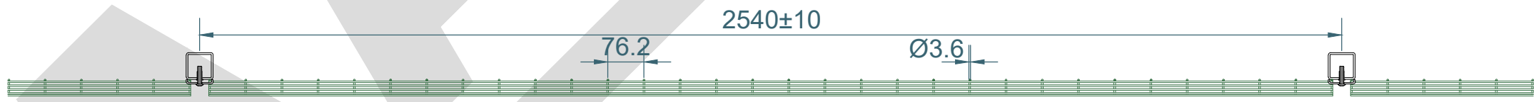
1-1 Section 1:12
