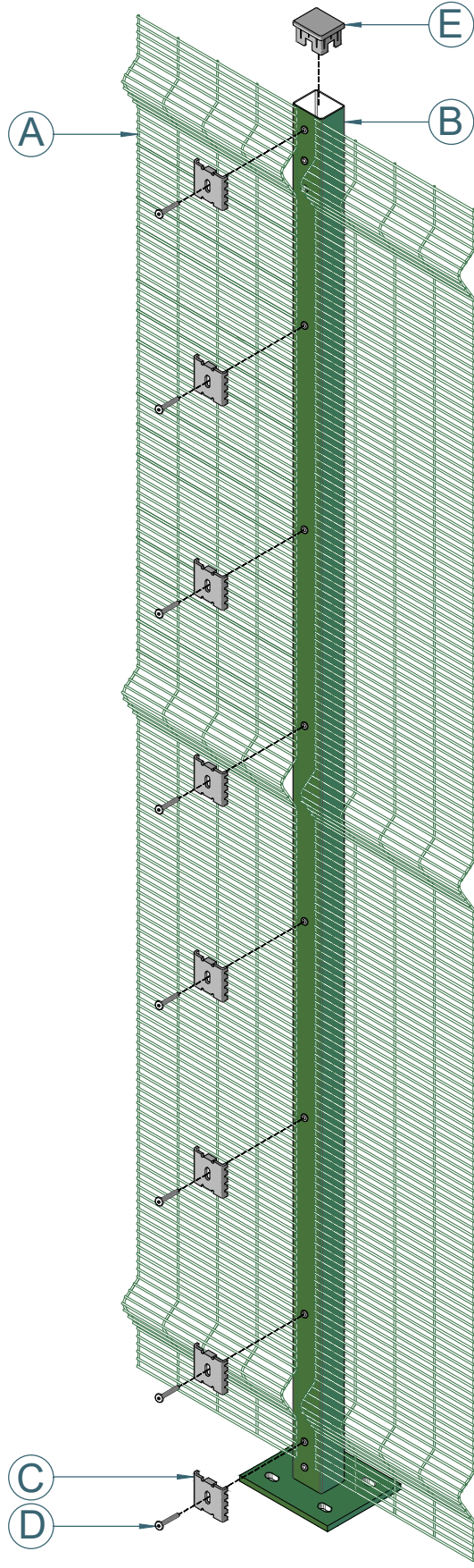
Axonometric Drawing
