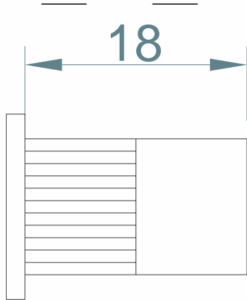
M8*18mm STAINLESS STEEL SECURITY NUT
