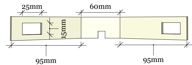
FISH PLATE CORNER
