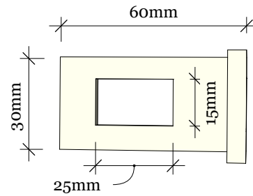
END FISH PLATE
