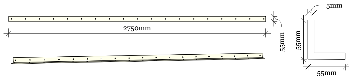
STEEL PALISADE BACK RAIL
