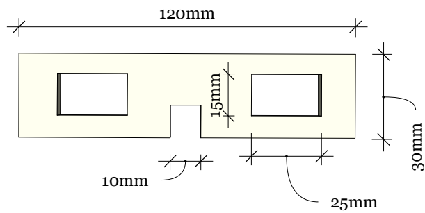
STRAIGHT FISH PLATE
